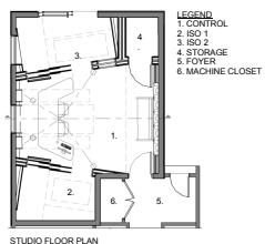
STUDIO FLOOR PLAN
