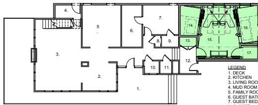
GROUND LEVEL FLOOR PLAN - RESIDENCE 0 2 4 6 8 10 20 FEET 0 1 2 3 6 METERS
