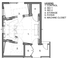
STUDIO FLOOR PLAN
