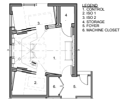
STUDIO FLOOR PLAN
