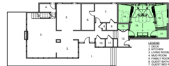
GROUND LEVEL FLOOR PLAN - RESIDENCE
