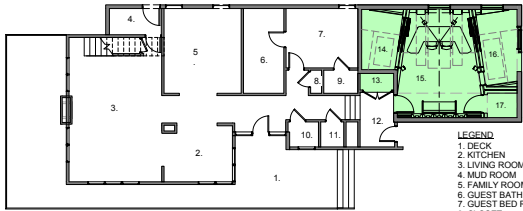
GROUND LEVEL FLOOR PLAN - RESIDENCE
