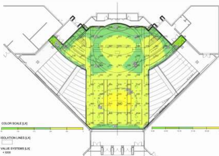
Photometric Plan - Mode 1
